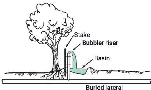
Figure 3. Basin Bubbler
