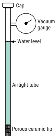
Figure 8. Tensiometer
