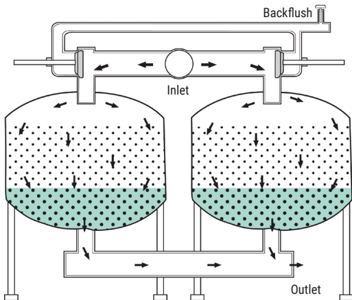
Figure 11. Media filter
